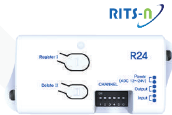
R24 (Receiver)
